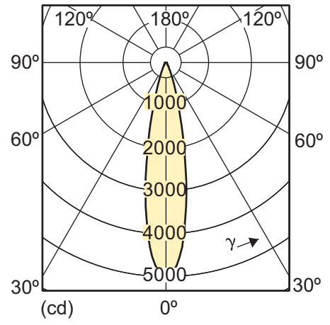
13-100 W E27 PAR38 /827 2700 K 25D
