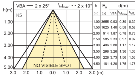
9.5-75W PAR30S 840 4000K 25D
