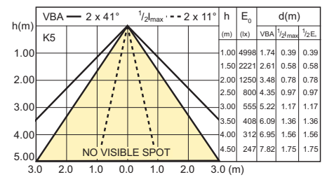
13-100 W E27 PAR38 /827 2700 K 25D
