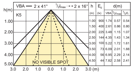
5.5-50W E27 2700K PAR20 40D
