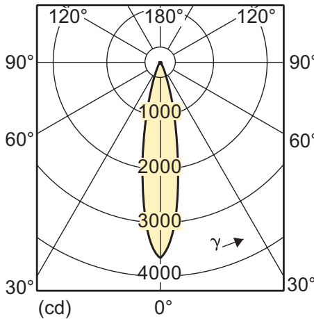
9.5-75W PAR30S 840 4000K 25D
