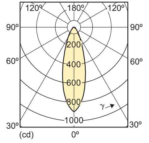
5.5-50W E27 2700K PAR20 40D
