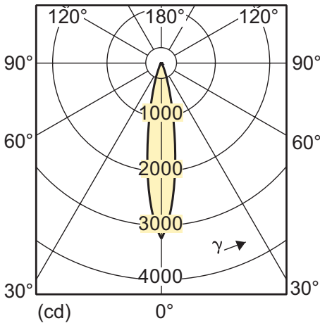
9.5-75W PAR30S 827 2700K 25D
