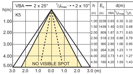
9.5-75W PAR30S 827 2700K 25D
