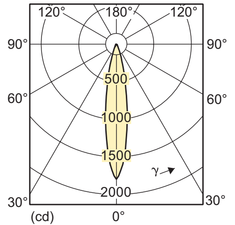
5.5-50W E27 2700K PAR20 25D
