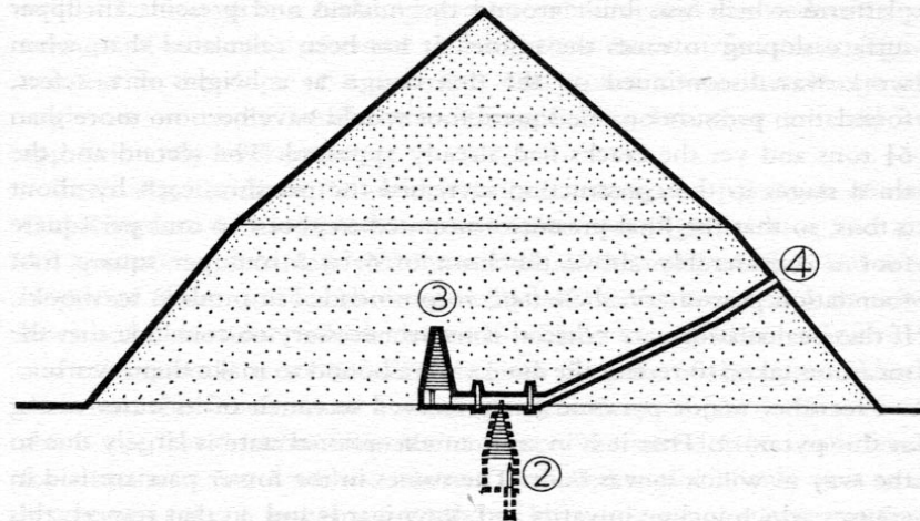
Figure 20. The Bent Pyramid, section looking south
