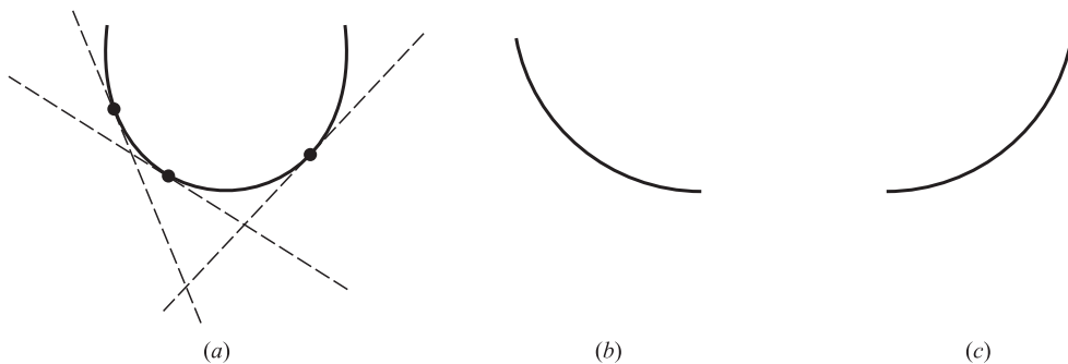
Fig. 23-1 Concavity upward
