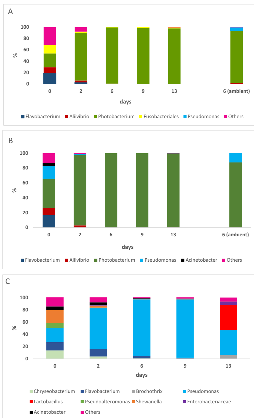
Fig. 2. The distribution of bacterial OTUs in products from two farms of salmon (A, B) and tuna (C) stored at 3 °C under vacuum, unless otherwise stated, based on 16S rRNA amplicon sequencing. Depending on the diversity of the 16S rRNA gene sequences, classification results are shown either at the genus or family level. Data are expressed as the mean of 2–3 replicates, except ambient atmosphere in day 6, which represents only one. Average percentages above 5% are plotted.
