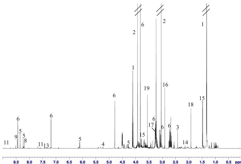
Fig. 3. Representative ^1\text{H} NMR spectrum of a tuna (A) and salmon (B) sample (day 13) with numbers indicating assignments.
