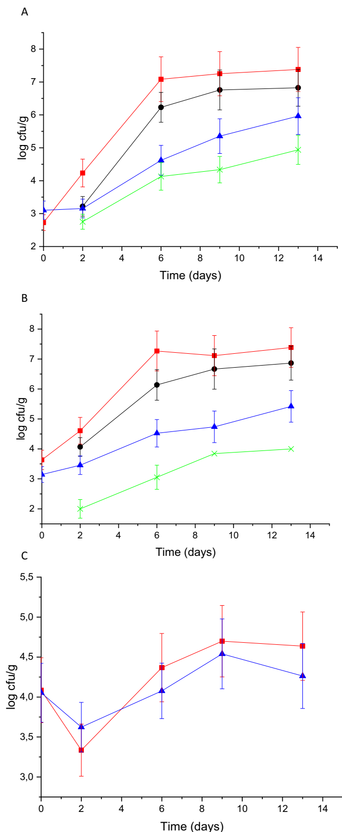
Fig. 1. Bacterial counts and growth curves: psychrotrophic (red square), bioluminescent (black circle), total (blue triangle) and sulphur producing bacteria (green cross) in Atlantic salmon from two farms (A, B) and Yellowfin tuna (C) stored under vacuum at 3^\circ\text{C} determined by plating. Data reported are mean values from three replicates, error bars represent standard deviation. (For interpretation of the references to color in this figure legend, the reader is referred to the web version of this article.)
