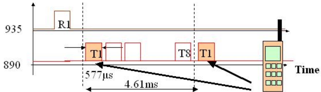
Time domain multiple access (TDMA)
