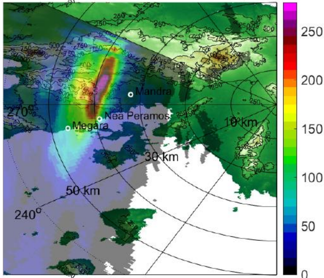
XPOL-NOA accumulated rainfall (mm)
