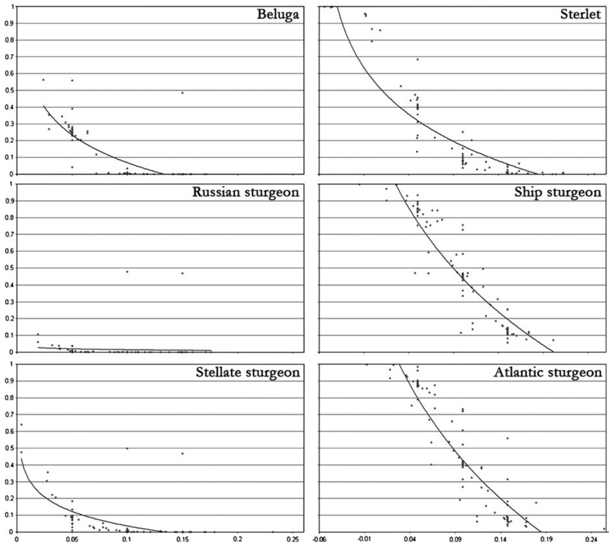
Fig. 1 Relationship between the deterministic population growth rate ( X axis) and the probability of pseudo-extinction ( Y axis) in the sensitivity analysis performed on the six Danube
