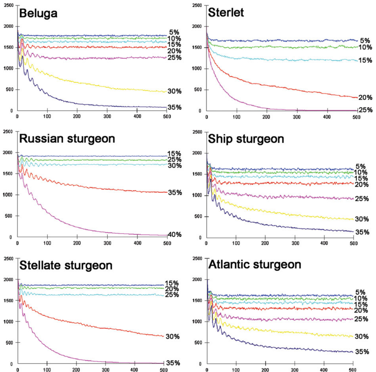
Fig. 5 Result of different harvest pressures applied on the six studied Danube sturgeon species (population growth rate r = 0.10 ). Y axis—average population size among all iterations in a simulation; X axis—years of the simulation; percentage
