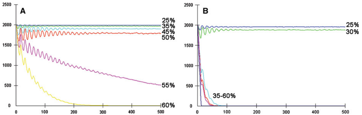
Fig. 6 Result of different harvest pressures applied on the Russian sturgeon (population growth rate r = 0.15 ). a Harvest of adults only; b harvest of both adults and the two oldest subadult age groups; Y axis—average population size among
