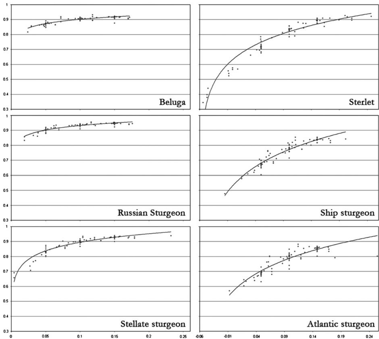
Fig. 2 Relationship between the deterministic population growth rate (X axis) and the expected heterozygosity (Y axis) in the sensitivity analysis performed on the six Danube
