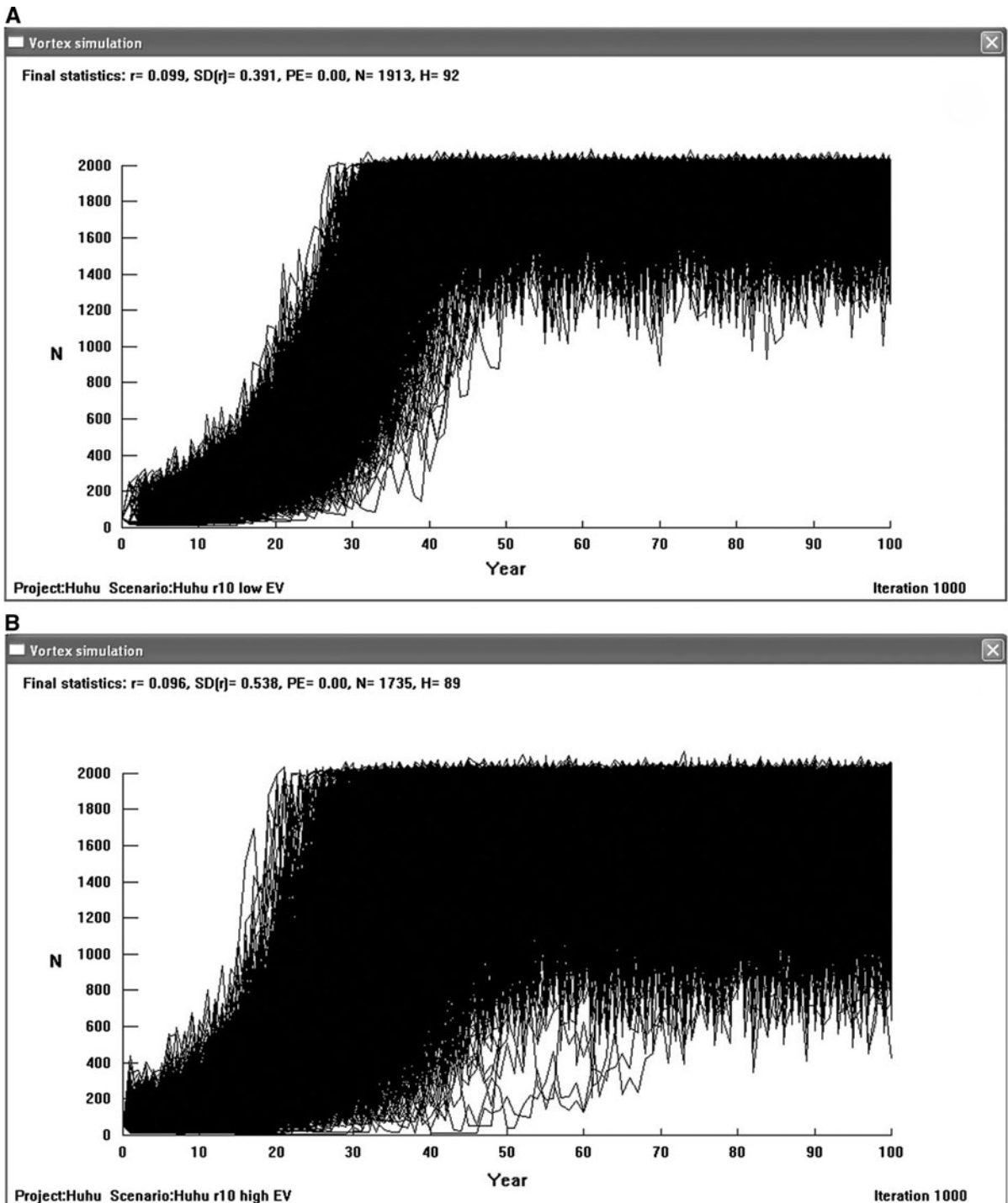
Fig. 3 Two scenarios with identical input data, except the larger amount of environmental variation that was applied in the scenario B. Images represent simulation screens from the Vortex program, with 1,000 iterations simulated in each scenario and population growth rate r = 0.10 . a All
