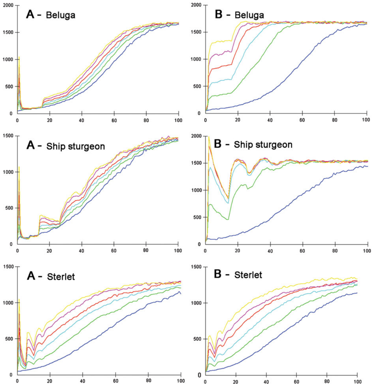
Fig. 7 Recovery of a small population of beluga, ship sturgeon and sterlet with different number of juvenile (a) or adult (b) individuals released in the first year of the simulation (population growth rate r = 0.05 ). From the lowest to the highest one, respectively, full lines in each graph represent: a the basic scenario and the release of 200, 400, 600, 800 and
