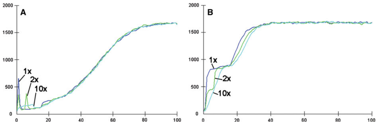
Fig. 8 Recovery of a small population of beluga, with the same number of juvenile (a) or adult (b) individuals released in three different patterns (population growth rate r = 0.05 ). 1x—All individuals released at once in the first year of the simulation, 2x—equal portions of individuals released two times, in the first and sixth year of the simulation, 10x—equal
