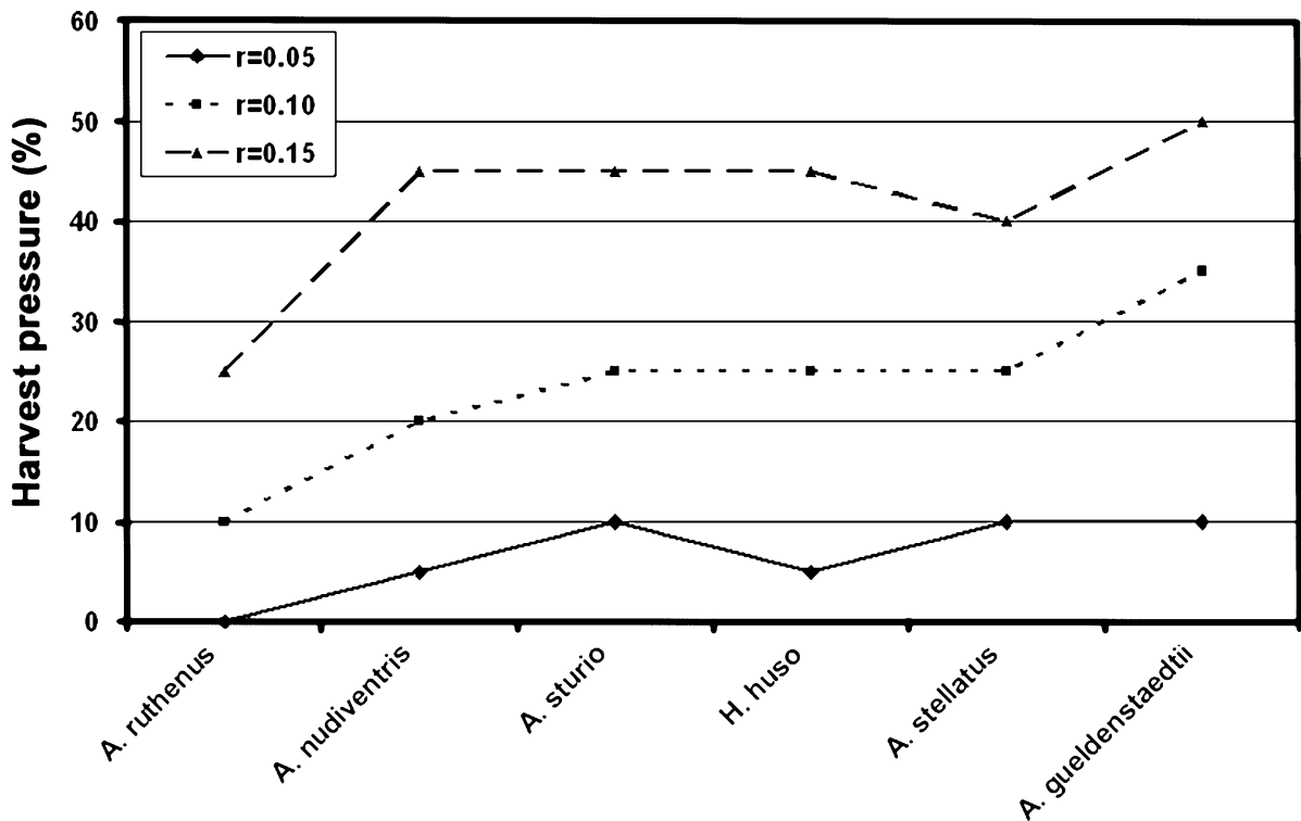
Fig. 4 Maximum harvest pressures at which the populations of six studied Danube sturgeon species remained viable (pseudo-extinction probability P < 0.05 ), given three different population growth rates ( r = 0.05, 0.10 and 0.15 )
