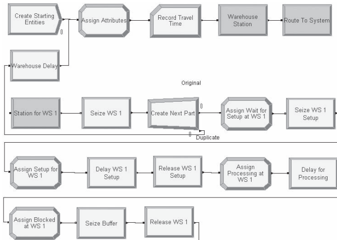
Figure 9-8. Part Arrival and Workstation 1
